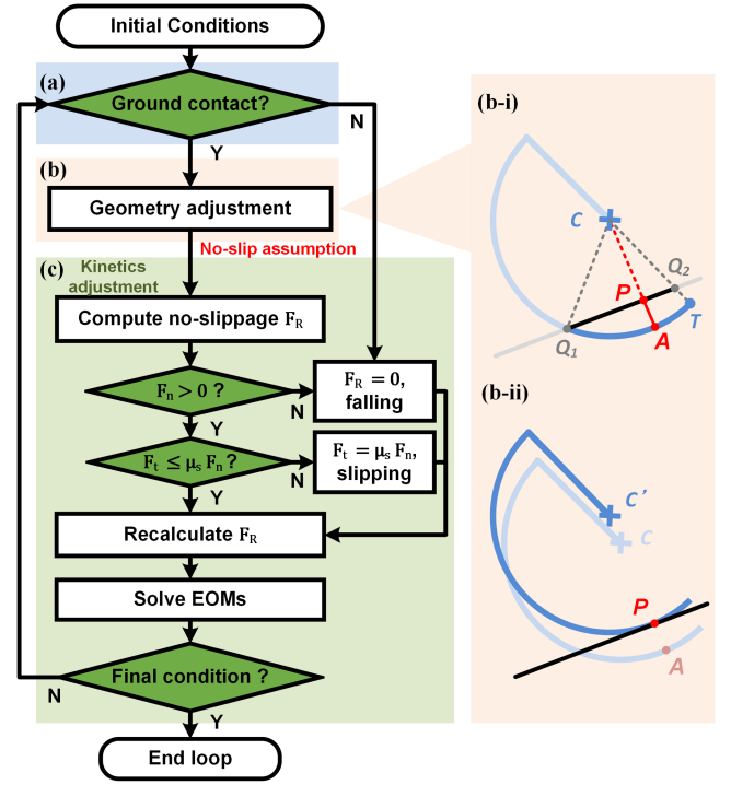
Fig. 5. Flow chart of the computational simulation of the dual-leg-wheel model. The three blocks in different colors refer to the three checks/adjustments. (a) Contact condition check. (b) Geometry adjustment. (c) Kinetics adjustment.
